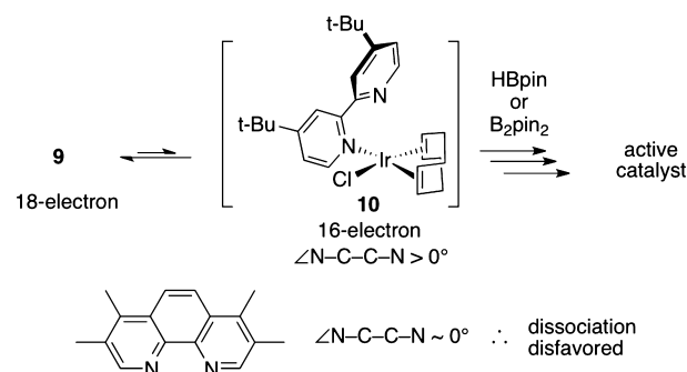
Scheme 4. Accessibility of κ 1 -Intermediates for Dipyriddy and Phenanthroline Ligands
