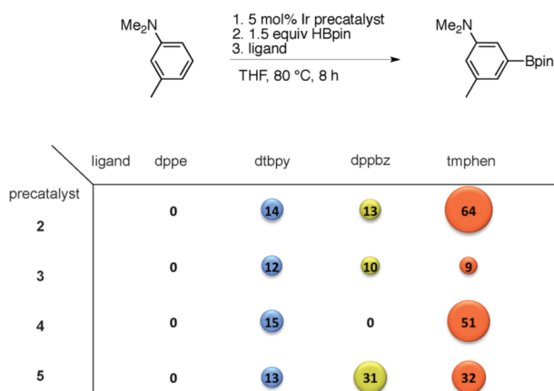
Figure 4. Comparison between dipyridyl and diphosphine ligated catalysts. Data plotted are product yields determined by HPLC. Results for dtbpy and tmphen are the same as shown in Figure 3.
