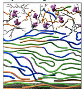
Layered fungal cell wall
