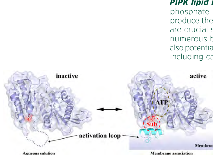
Figure 3. Activation loop (cyan) acts as a membrane sensor governing the activity of PIPKs.
