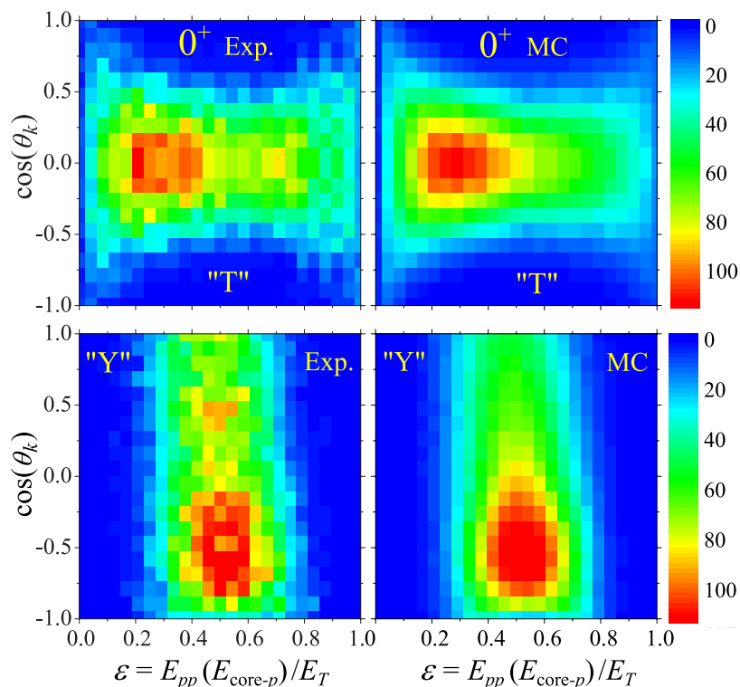
Energy-angular correlations for the two-proton decay of the ground state of ^{16}\text{Ne} . The experimentally measured distributions (left) are compared to a three body model prediction adjusted for detector resolution (right).
