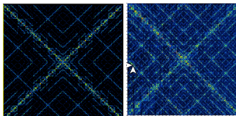
Theory (left), experiment (right) demonstrating selective vibrational excitation of molecules by stimulated Raman excitation using binary shaped pulses.
