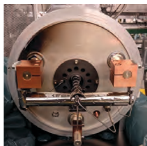
32 Si ion source (left) to facilitate the stand-alone operation of the ReA-facility. The ion sources are introduced into the Batch Mode Ion Source module (right).
