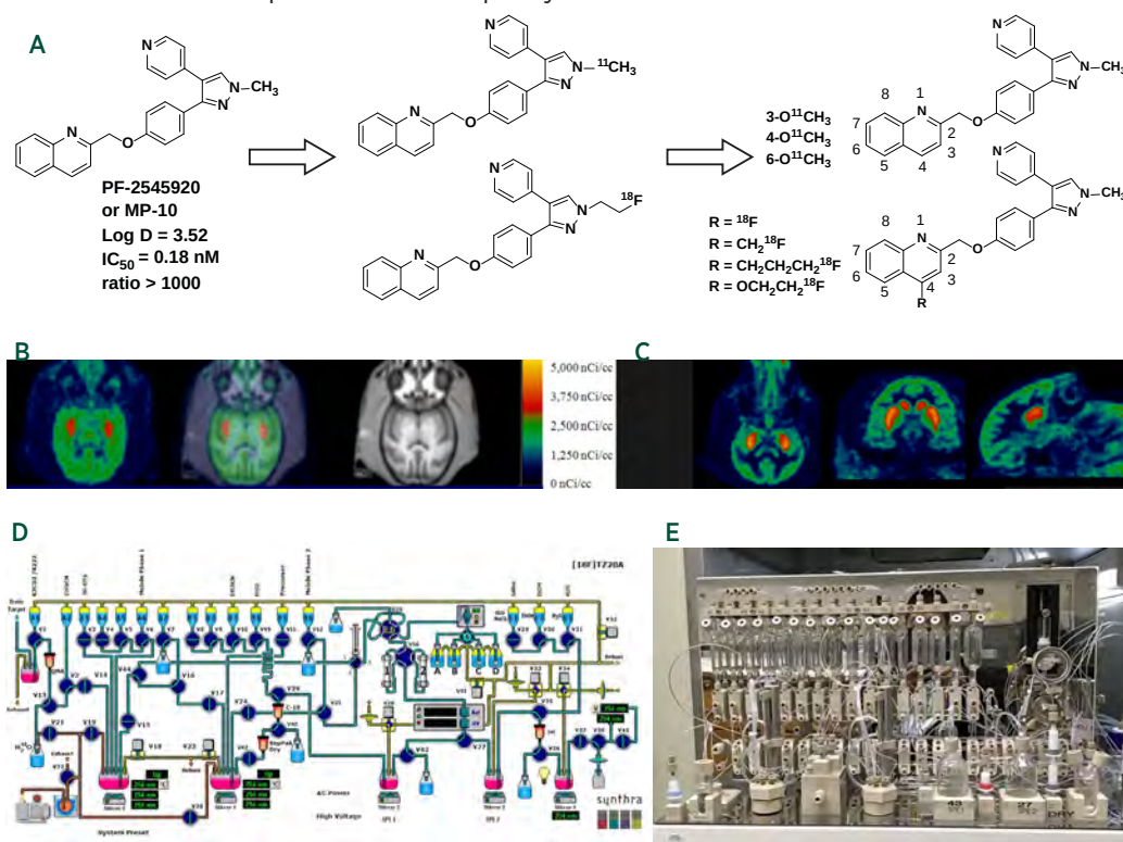
A) A scheme demonstrates the development of 18 F and 11 C PET radiotracers for PDE10A, from MP-10, a potent and highly selective PDE10A inhibitor, the first generation of tracers were labeled on the pyrazole moiety, and to improve metabolic stability, the second generation tracers were labeled on the quinoline moiety. B) PET imaging results of Rhesus monkeys using [ 11 C]MP-10, a representative summed image from 0 to 120 min is overlay with MRI images to accurately identify the regions of interest, caudate and putamen. C) Representative summed image of [ 18 F]FEMP-10, axial, coronal, and sagittal images of a monkey's brain. D) A program chart displays the work flow on an automated synthesis module. E) A picture of the synthesis module, on which the radiolabeling synthesis is conducted.
