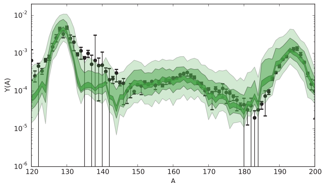
Predicted abundances as a function of mass number compared to solar r -process residuals (black dots). The shaded bands show the variances in a large number of predicted abundance patterns taken from network calculations. In each calculation a variation of all neutron capture rates is applied. The shaded bands correspond to neutron capture rate uncertainties of a factor of 100 (light), 10 (middle), and 2 (dark). All but the largest abundance pattern features are obscured by the rate uncertainties at a factor of 100. Only with uncertainties smaller than a factor of 10 can fine features be observed.
