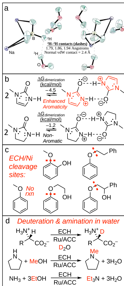
Figure 1. (a) Structure of NaBD_4 \cdot 2D_2O showing close D...D contacts of three D_2O molecules to one BD_4^- deuteron; (b) Aromaticity-enhanced H-bonds vs. localized reference; (c) Surprisingly diverse ether bond cleavages promoted by mild (60 °C, aqueous electrolyte, skeletal Ni cathode) electrocatalytic reduction; (d) Mild aqueous electrocatalytic C-H activation and halide-free amination using simple alcohols.
