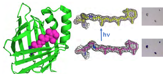
Left , The structure of a retinal-bound hCRABPII variant. Right , pictures of crystals of an hCRABPII variant before (top) and after (bottom) UV irradiation. Center , the electron density map of retinal bound to an hCRABPII variant before (top) and after (bottom) irradiation with UV light showing specific photoisomerization in the single crystal that gives rise to the color change.
