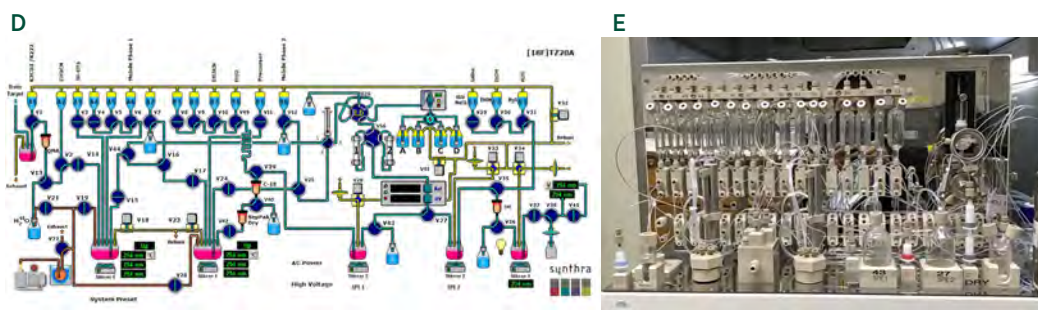
A) A scheme demonstrates the development of 18 F and 11 C PET radiotracers for PDE10A, from MP-10, a potent and highly selective PDE10A inhibitor, the first generation of tracers were labeled on the pyrazole moiety, and to improve metabolic stability, the second generation tracers were labeled on the quinoline. B) PET imaging results of Rhesus monkeys using [ 11 C]MP-10, a representative summed image from 0 to 120 min is overlay with MRI images to accurately identify the regions of interest, caudate and putamen. C) Representative summed image of [ 18 F]FEMP-10, axial, coronal, and sagittal images of a monkey's brain. D) A program chart displays the work flow on an automated synthesis module. E) A picture of the synthesis module, on which the radiolabeling synthesis is conducted.
