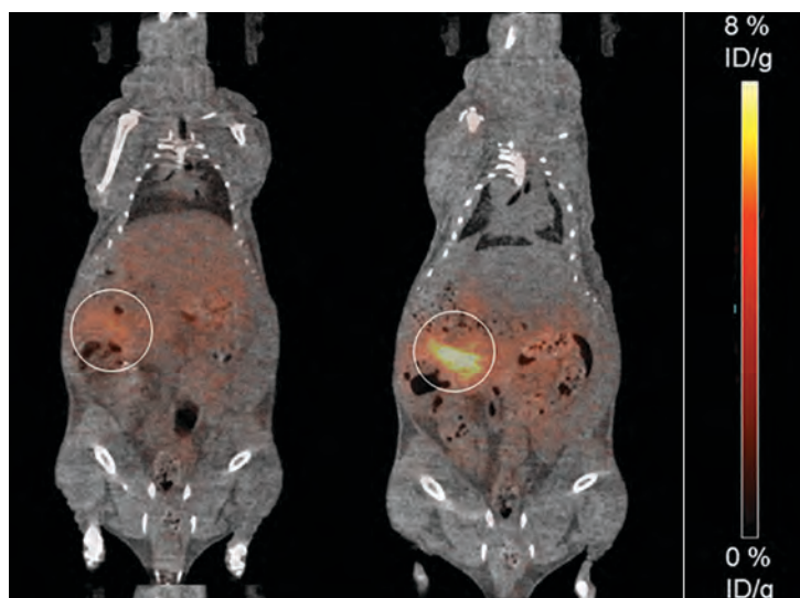
Figure 1: (left) Pre- and (right) post-mortem PET/CT scan of a mouse 16h after injection with a somatostatin receptor 2 (sst2+) targeting peptide, DOTA-LM3, labeled with ^{140}\text{Nd} . The white circle is drawn over the pancreas (sst2+) where the difference in the pre- and post-mortem pancreatic signal is due to rapid diffusion of ^{140}\text{Nd} 's short-lived daughter nuclide, ^{140}\text{Pr} , from the highly perfused pancreas into the blood stream. With further development, similar techniques with ^{140}\text{Nd} may be used to determine the in vivo internalization status of labeled therapeutics.
