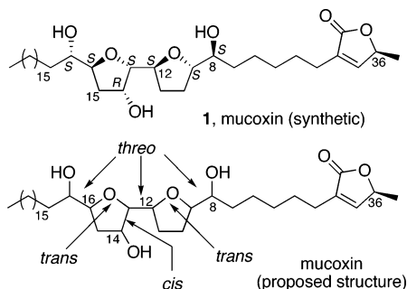
FIGURE 6. Structure of synthetic mucoxin ( 1 ) and proposed mucoxin.
