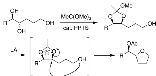
FIGURE 2. Revised retrosynthesis for construction of the disubstituted THF ring.
