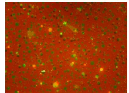
Molecular-scale information
